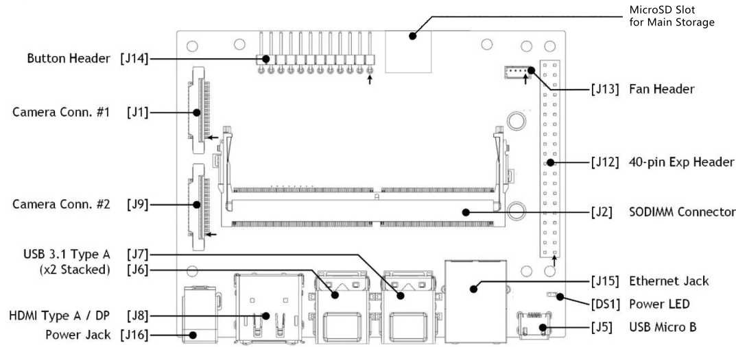
Top view of Development System carrier board
